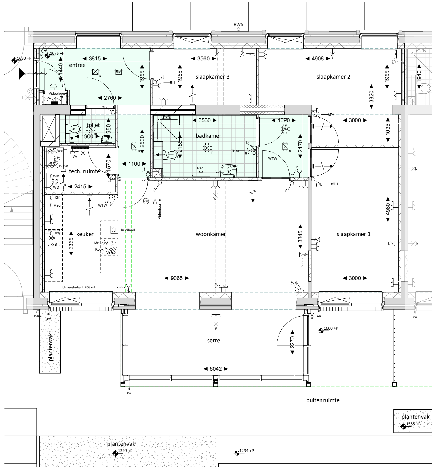
00 begane grond
