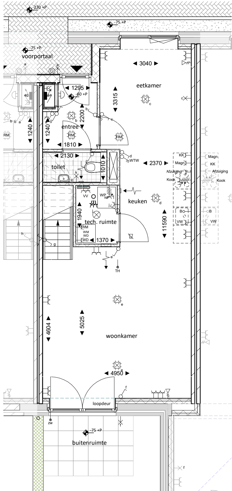
00 begane grond
